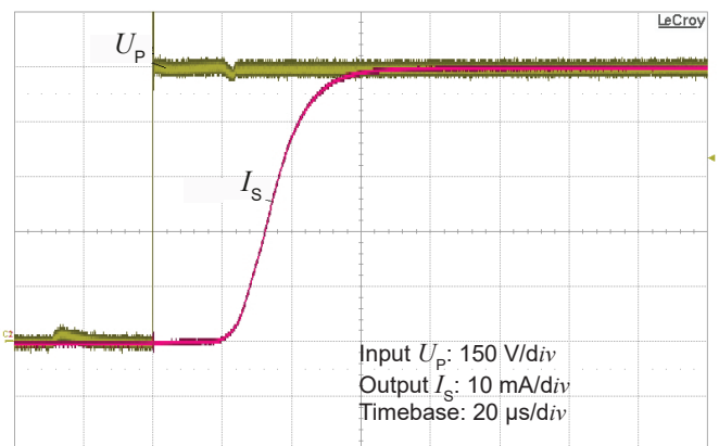
Figure 6: Typical step response (0 to 750 V)
