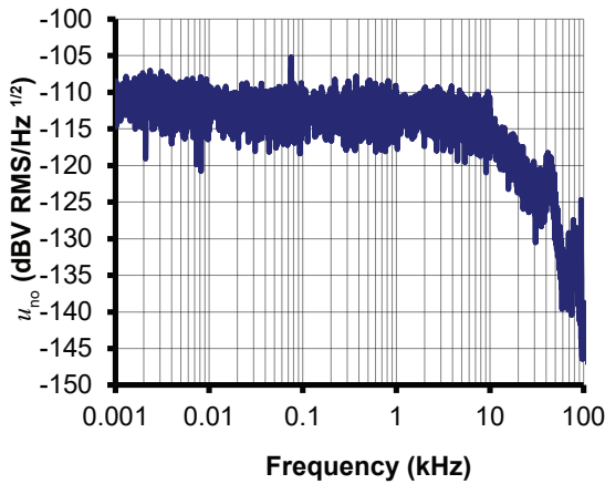
Figure 15: Typical output RMS noise voltage spectral density u_{no} with R_M = 50 \Omega
