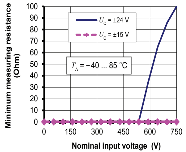
Figure 2: Minimum measuring resistance The derating @ \pm 24 V is only applicable for T_A = 80 \dots 85^\circ\text{C} For T_A under 80^\circ\text{C} , the minimum measuring resistance is 0\ \Omega whatever U_C
