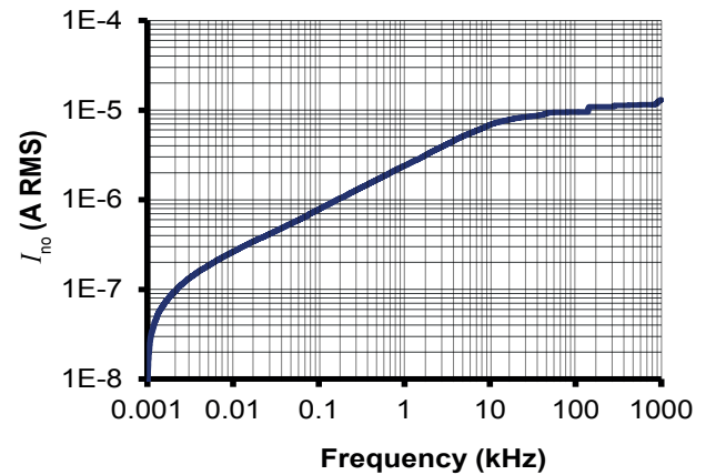
Figure 16: Typical total output RMS noise current with R_M = 50 \Omega
