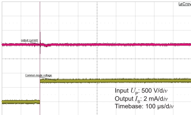
Figure 13: Typical common mode perturbation (750 V step with 6 kV/μs R_M = 100 \Omega )
