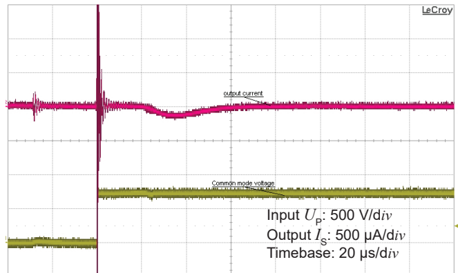
Figure 14: Detail of typical common mode perturbation (750 V step with 6 kV/μs, R_M = 100 \Omega )
