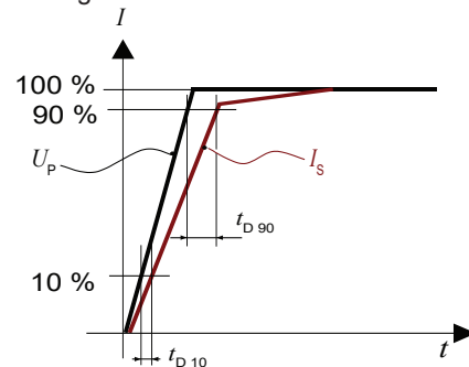
Figure 19: Delay time t_{D90} @ 90 and delay time t_{D10} @ 10
